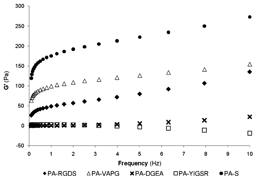
Figure 2. Measure of storage modulus ( G' ) over frequency using dynamic oscillatory rheometry. Individual PAs exhibited different viscoelastic properties after induced self-assembly.
